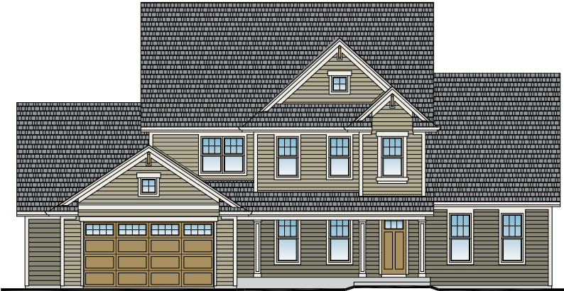
Elevation II
